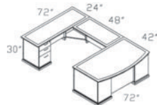
EM6902L/R EXECUTIVE 'U' W/BOW TOP DESK EM6902L.R.MAHO-MAHOGANY EM6902L/R.MAP-MAPLE (EM6902L SHOWN)
