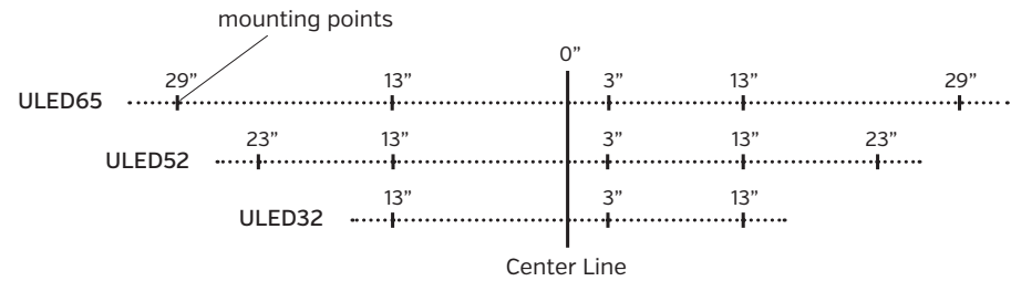
Mounting Diagram
